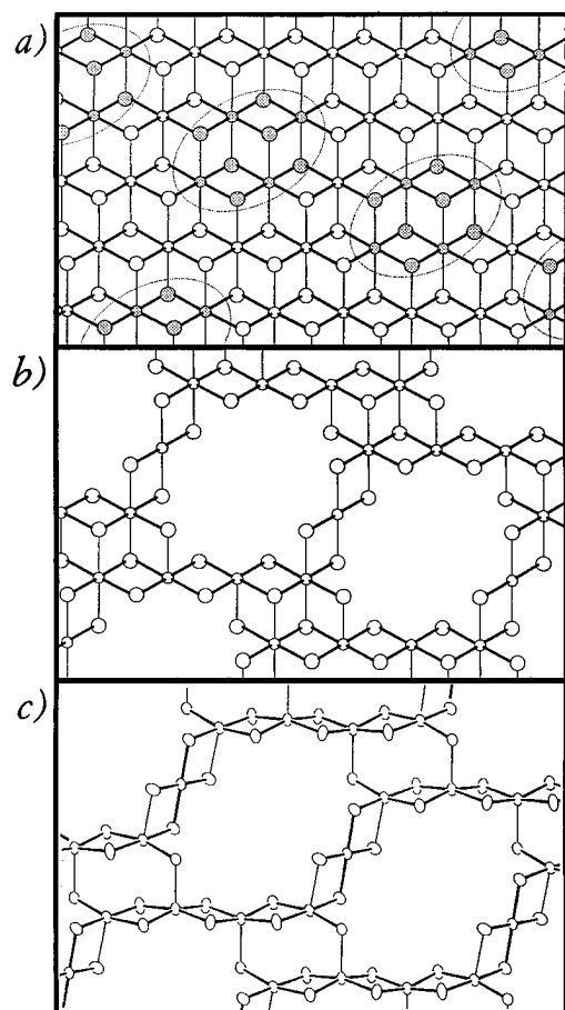
Figure 3. Relation of the chlorocuprate structure in [(C 2 H 5 ) 4 N] 2 Cu 5 Cl 12 to the parent CuCl 2 structure: Cl, larger circles; Cu, smaller circles. Key: (a) Representation of the CuCl 2 structure, with bibringed chains running horizontally. Semicoordinative linkages between chains are visualized by vertical dashed lines. The dotted ellipsoids mark the (Cu 4 Cl 6 ) 2+ fragments that must be removed to generate the [(Cu 5 Cl 12 ) 2- ] ∞ network structure. (b) Ideal structure after removal of (Cu 4 Cl 6 ) 2+ fragments from the CuCl 2 network. (c) Real chlorocuprate network in the [(C 2 H 5 ) 4 N] 2 Cu 5 Cl 12 structure.
