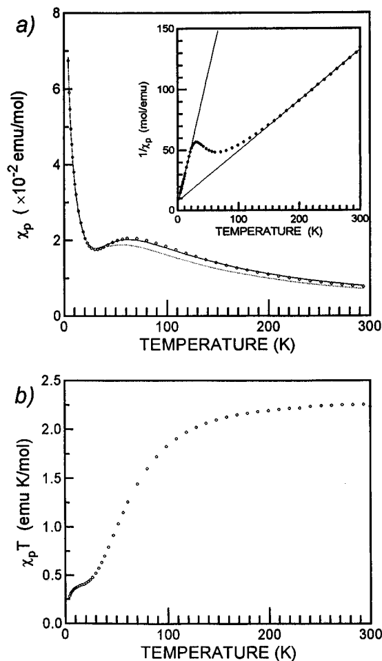
Figure 4. Experimental paramagnetic susceptibility, \chi_p , of [(C 2 H 5 ) 4 N] 2 Cu 5 Cl 12 (a) and the \chi_p T product (b) as a function of temperature. The line in part a is the best fit of eq 1 (see text); the inset shows the plot of \chi_p^{-1} vs T .
